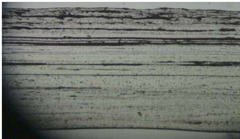
Section of a HDPE Container Wall with KORTRAX® Barrier Layers
